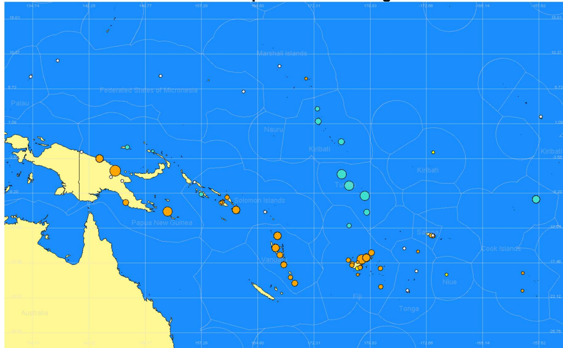
Legend ● Bias towards below-normal rainfall ● Bias towards normal rainfall ● Bias towards above-normal rainfall No bias in forecast (Climatology) Larger "bubbles" represent higher forecast skill (based on LEPS scores)
