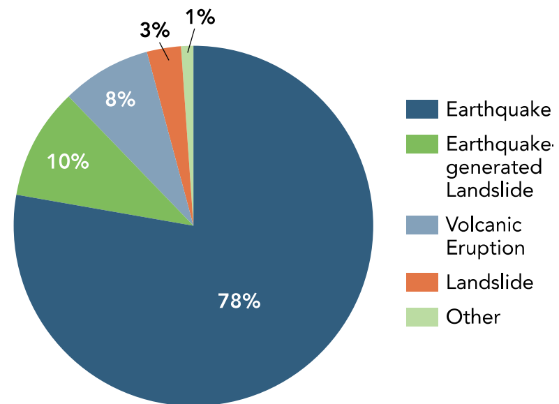
Distribution of causes for deadly Pacific tsunamis. Credit: NGDC
