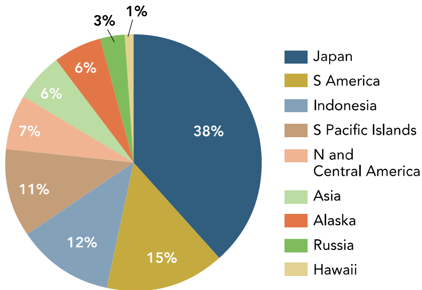
Geographic distribution of deadly Pacific tsunami sources. Credit: NGDC
